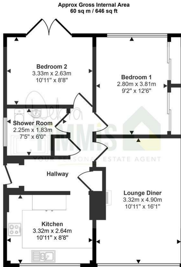
Floorplan
